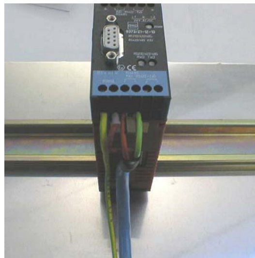
Fig 7 Connection of the external resistor
