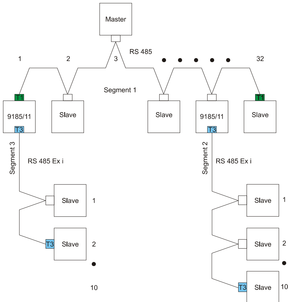
Fig 2 RS 485 Ex i conform to the R. STAHL specification with fieldbus isolating repeater type 9185
