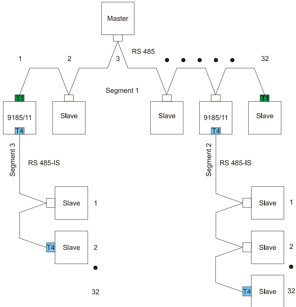
Fig 1 RS 485-IS conform to the PNO specification with fieldbus isolating repeater type 9185
