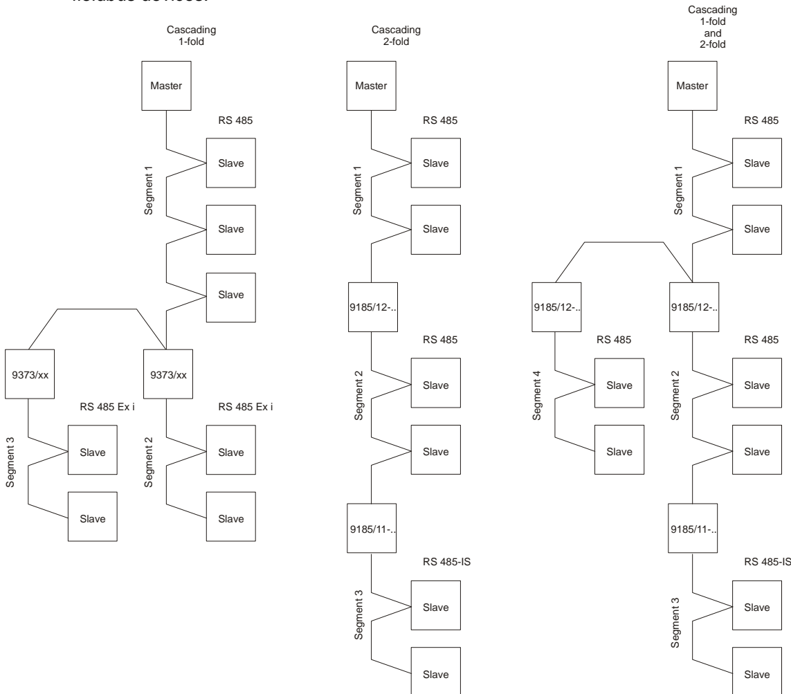
Fig 4: The illustration on the left indicates single cascading. There is a maximum of 1 type 9373/21... isolating repeater between the master and any slave. The illustration in the centre indicates double cascading. Two type 9185/.. fieldbus isolating repeaters are arranged between the master and the most distant slave. The right-hand illustration shows a combination of the two others.
