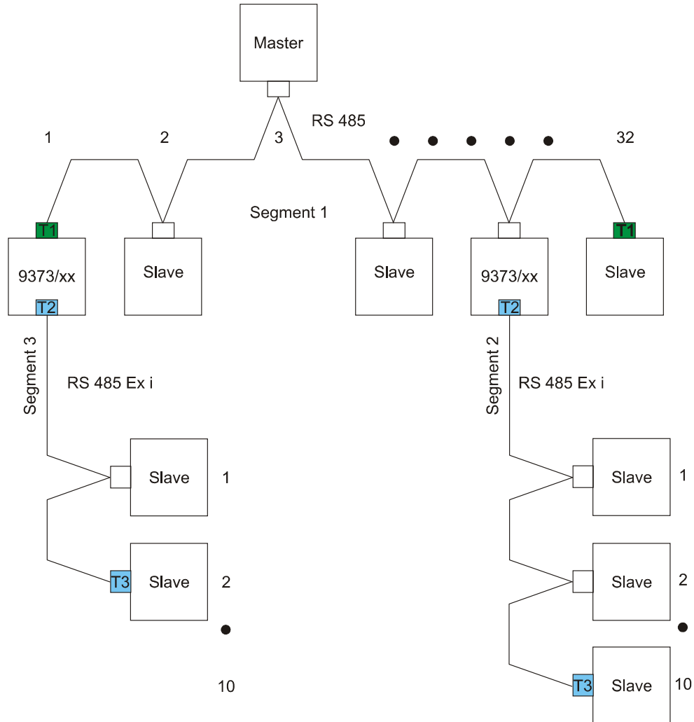
Fig 3 RS 485 Ex i conform to the R. STAHL specification with fieldbus isolating repeater type 9373
