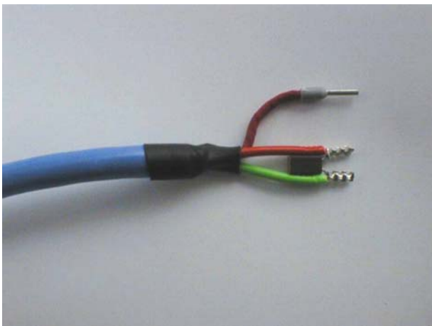
Fig 6 external 470 Ohm resistor
