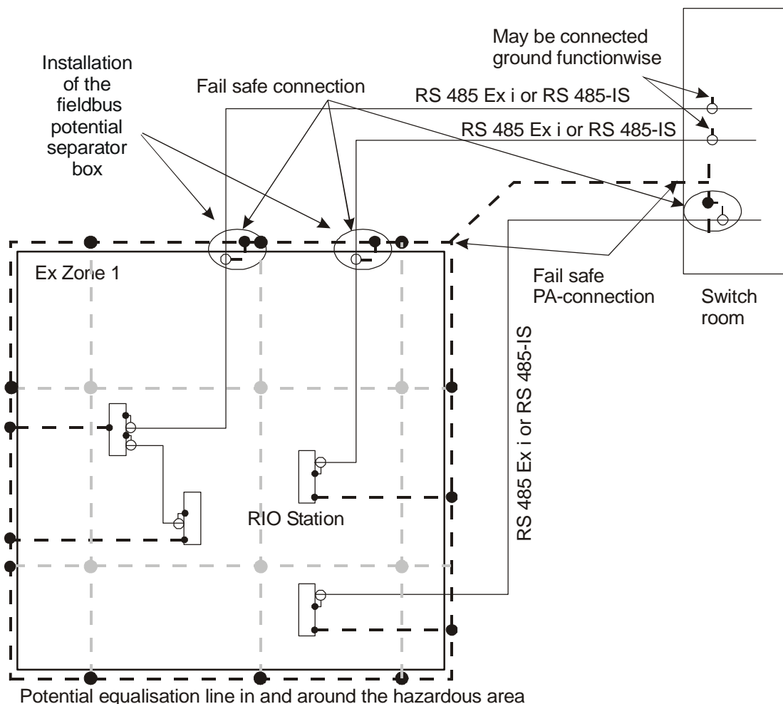
Fig 8 Earthing of a conductive shield
