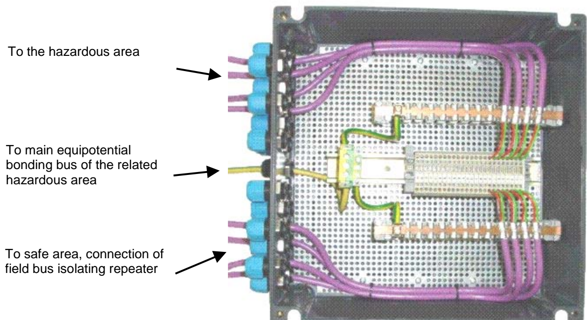
Fig 9 Example of a fieldbus potential isolating box
