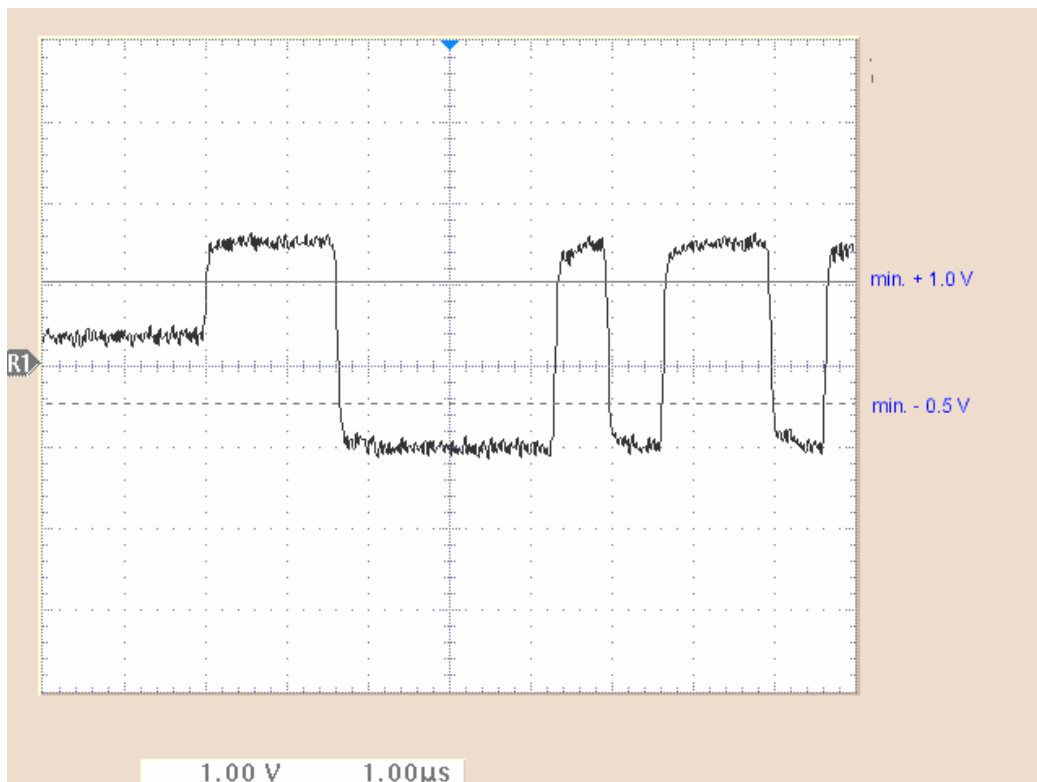
Fig 12 Minimum transmission levels on the RS 485 Ex i bus in accordance with R. STAHL Specification. The level should be above + 1 V and below – 0.5 V. The quiescent level is approx. 0.2 to 0.3 V in the case of a correctly terminated bus.
